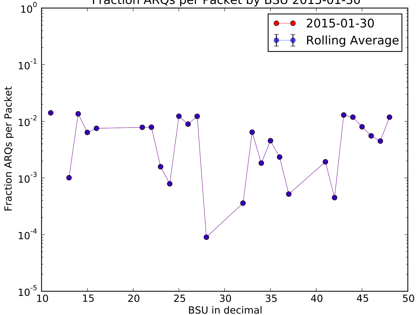
Fraction ARQs per Packet by BSU 2015-01-30
