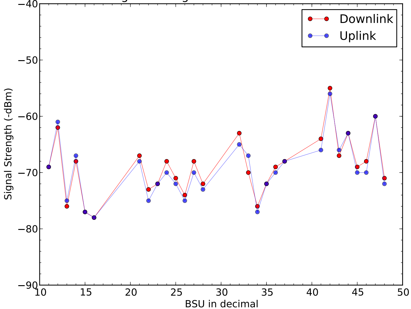
Signal Strength of BSU on 2015-01-23
