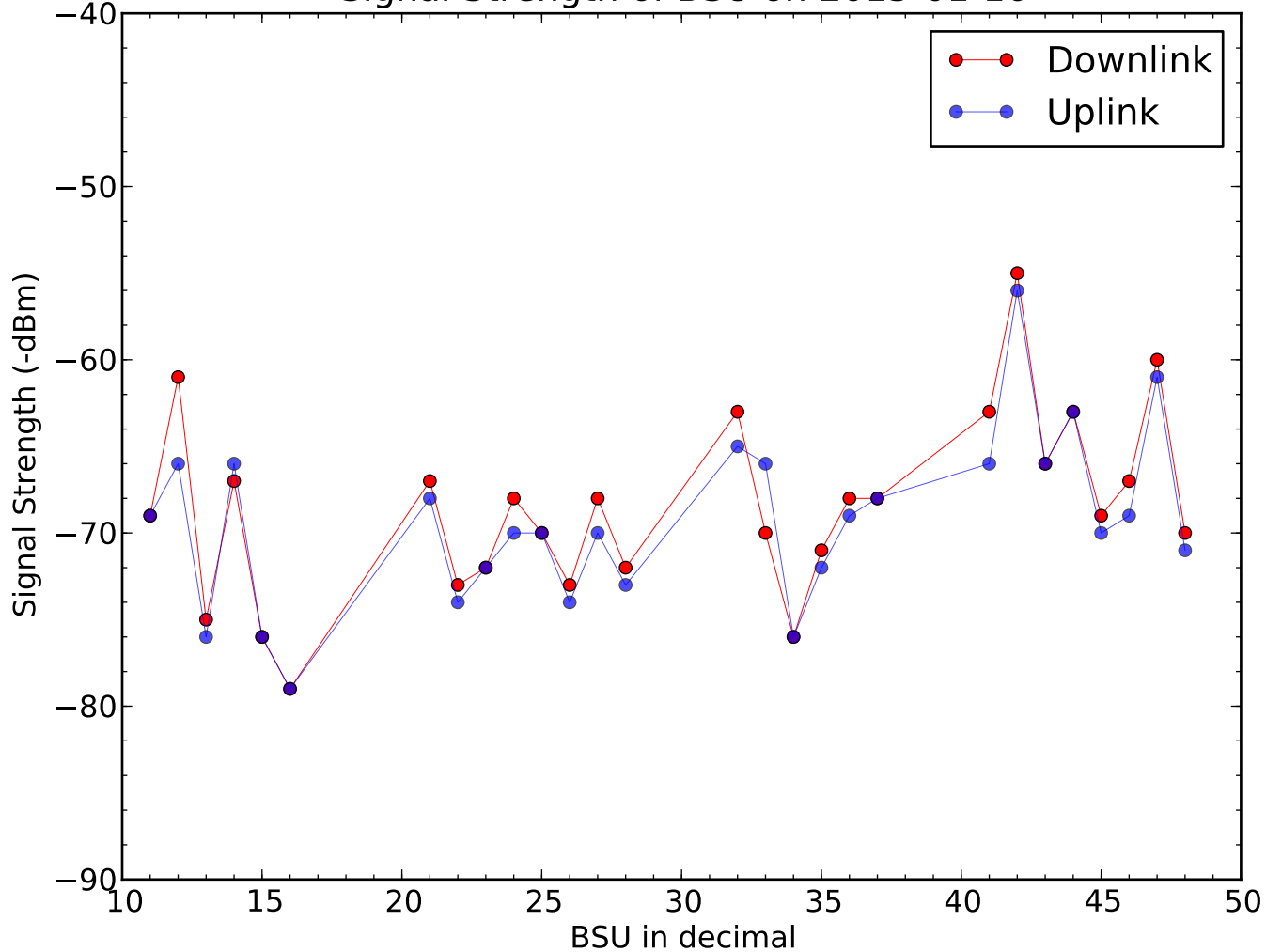
Signal Strength of BSU on 2015-01-16
