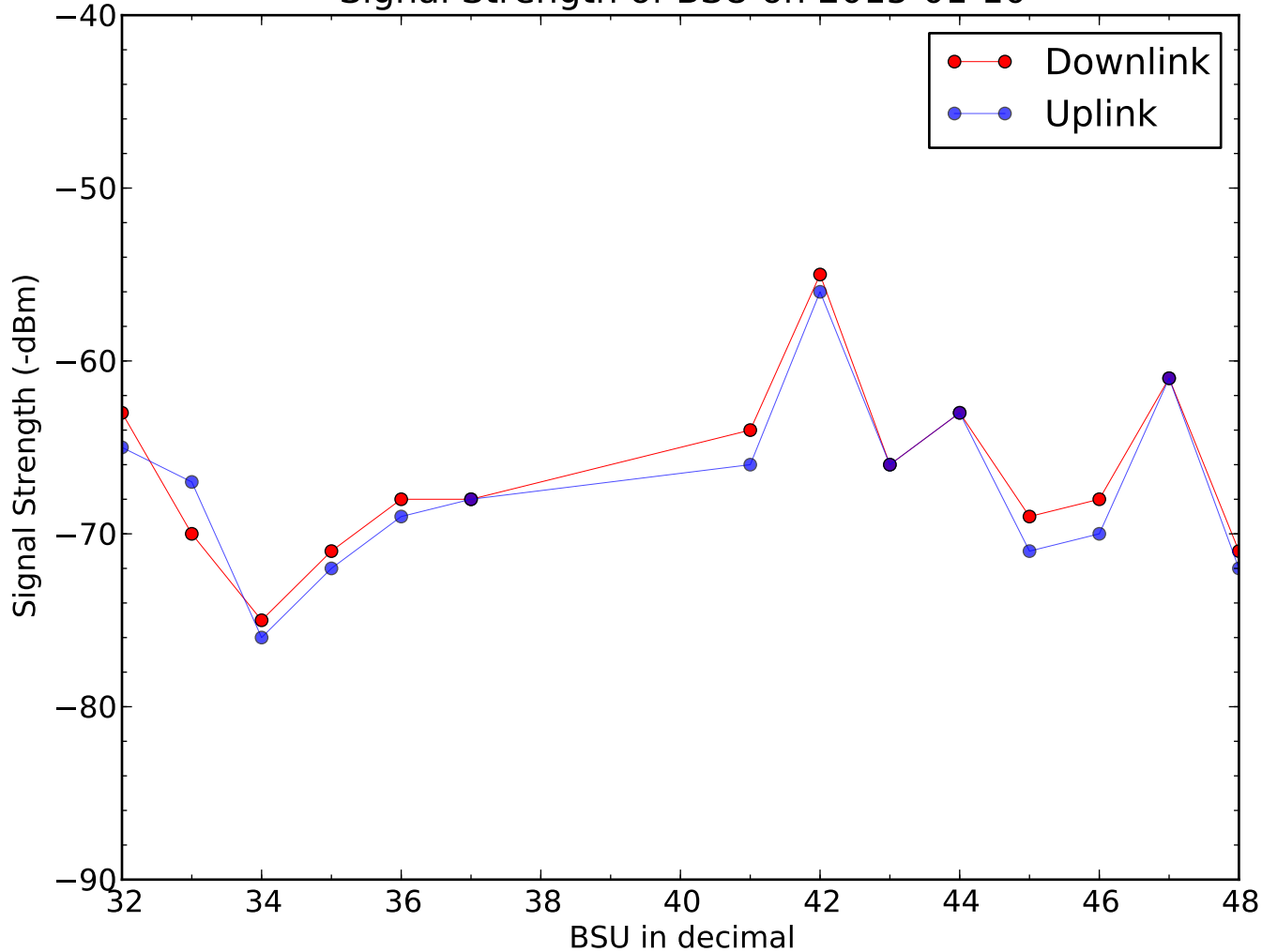
Signal Strength of BSU on 2015-01-10
