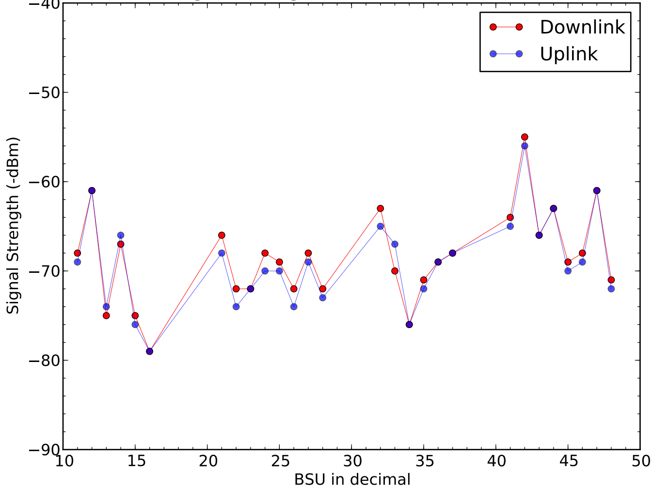
Signal Strength of BSU on 2015-01-04
