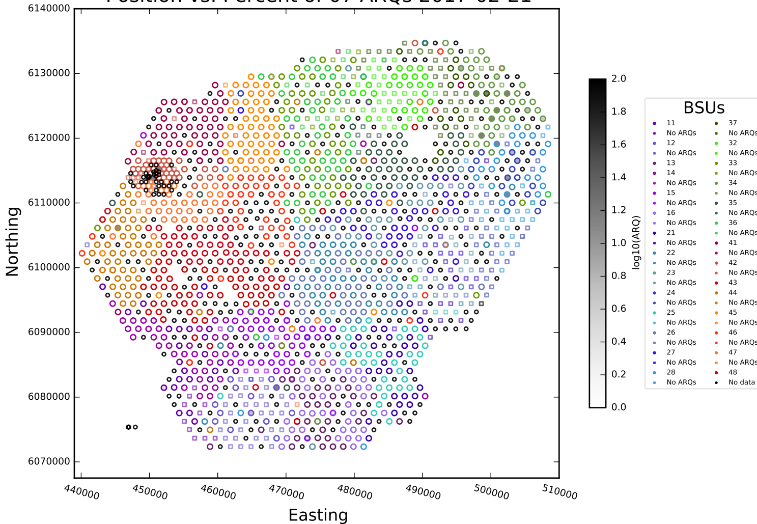
Position vs. Percent of 07 ARQs 2017-02-21
