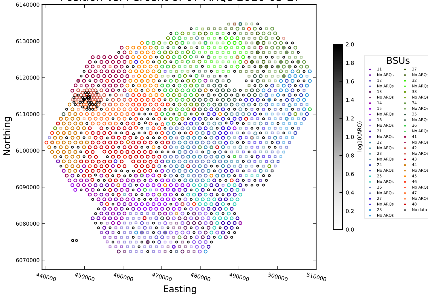
Position vs. Percent of 07 ARQs 2016-03-27
