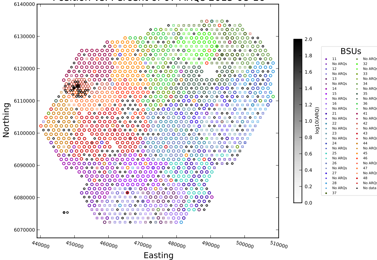
Position vs. Percent of 07 ARQs 2015-08-16
