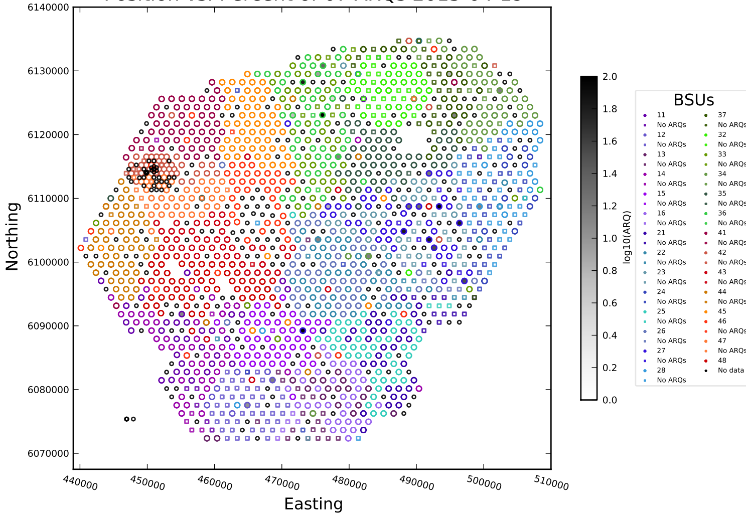
Position vs. Percent of 07 ARQs 2015-04-19
